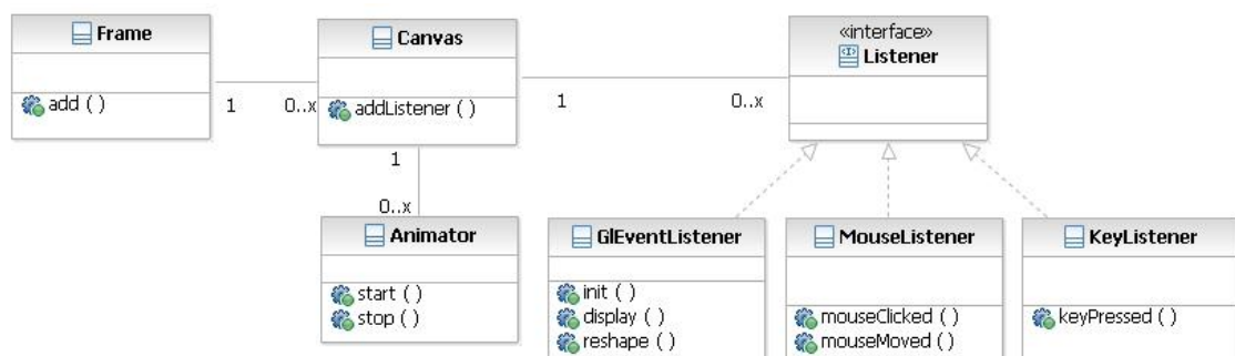
Figure 8 Classes JOGL
